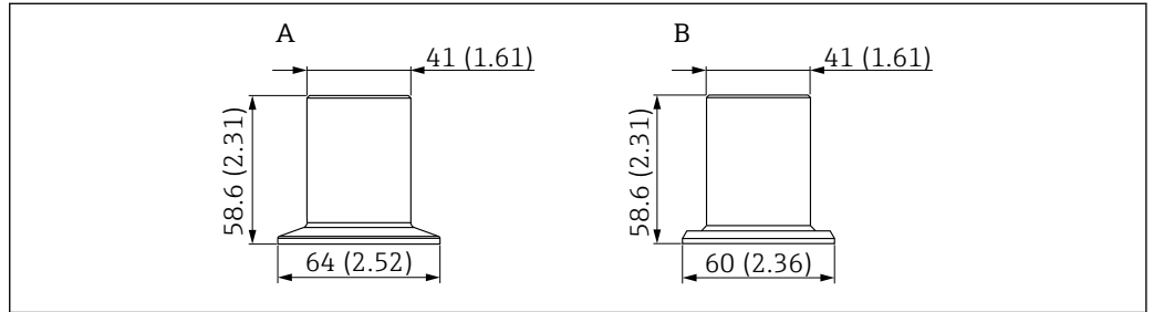
A Tri-Clamp 2", order code 620, option RI B Weld-in adapter G 1", order code 620, option PI
