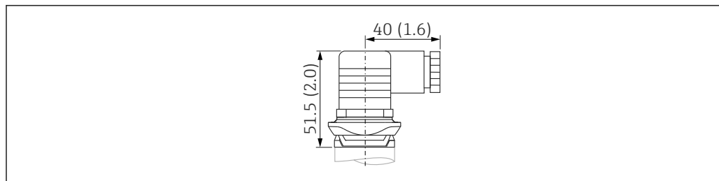
9 Valve plug M16, NPT 1/2"
